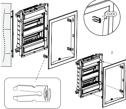
4 point connection
