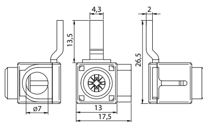
EFB-25PS-15
