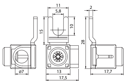
EFB-25FS-15
