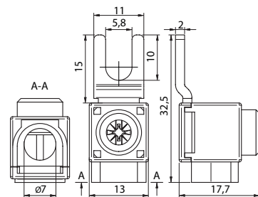
EFB-25FT-15
