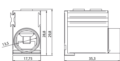
EFB50
