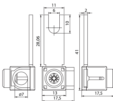
EFB-25FS-28
