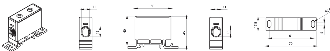
EDBS-50.., EDBS-50../N, EDBS-50../PE
