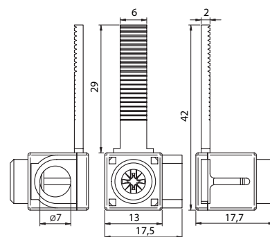
EFB-25PS-29
