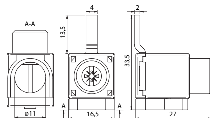
EFB-50PT-15
