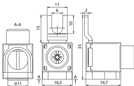
EFB-50FT-15
